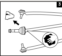
Remove old boot and clean joint.
